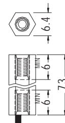
M3X0.5P BRASS NUT
