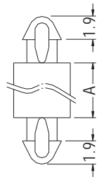
P.C.B Ø2.5 THICKNESS 1.6 FOR MADM-2~MADM-5
