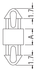
P.C.B Ø2.5 THICKNESS 1.6 FOR MADM-2.7S, MADM-3S
