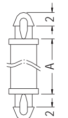
P.C.B Ø2.5 THICKNESS 1.6 FOR MADM-12.7
