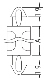
P.C.B Ø2.5 THICKNESS 1.6
