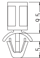
CHASSIS Ø4.8-Ø5.0 THICKNESS 0.8-2.0
