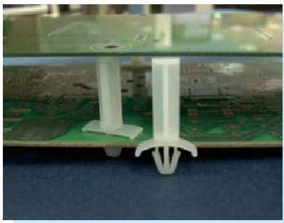
CHASSIS Ø4.8 THICKNESS 0.8-2.0
