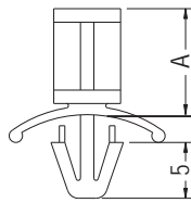
CHASSIS Ø4.8 THICKNESS 0.8-2.0
