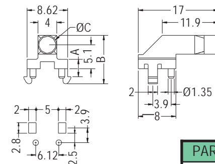
MOUNTING HOLES
