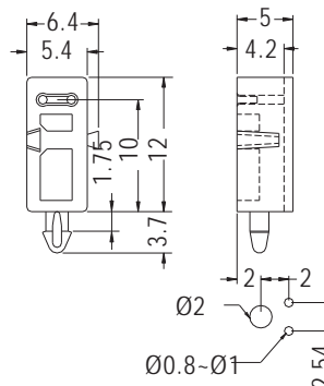
MOUNTING HOLES
