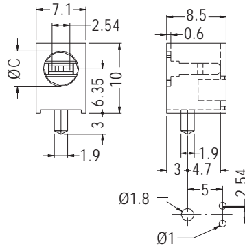
MOUNTING HOLES
