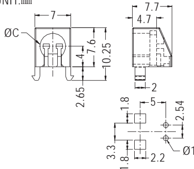
MOUNTING HOLES
