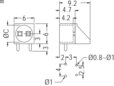
MOUNTING HOLES
