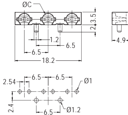
MOUNTING HOLES
