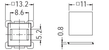
MOUNTING HOLE
