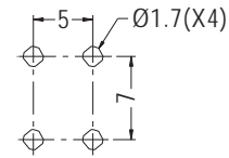
MOUNTING HOLES
