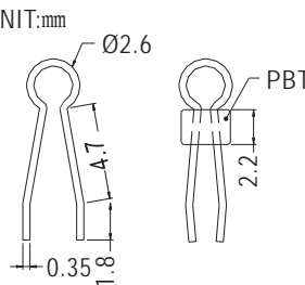
TEST-7 HOLE IN P.C.B Ø0.8-Ø1.0
