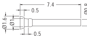
HOLE IN P.C.B Ø0.8~Ø0.9
