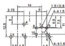
PC.B LAYOUT (VIEWED FROM COPPER SIDE)
