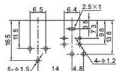
PC.B LAYOUT (VIEWED FROM COPPER SIDE)
