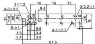
PC.B LAYOUT (VIEWED FROM COPPER SIDE)
