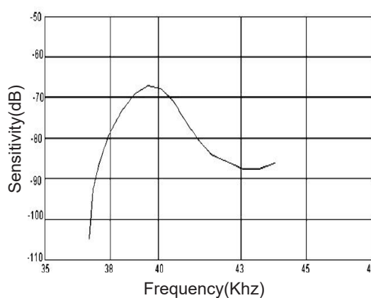
SPL-Frequency Characteristics
