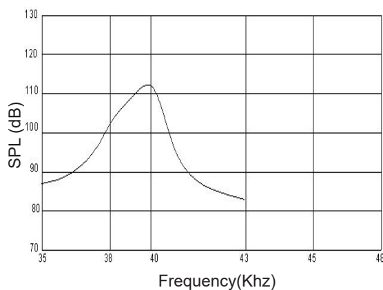
SPL-Frequency Characteristics
