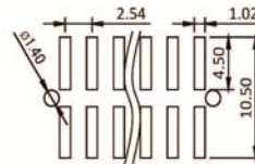
Recommended PCB Layout (PCB TOLERANCE ±0.05)
