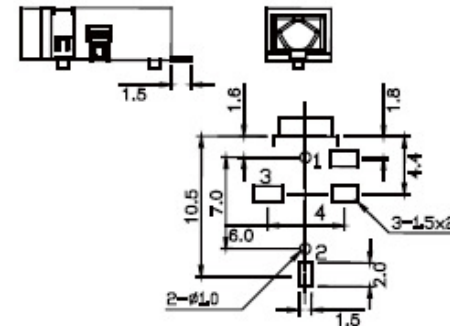
Recommended PCB Layout (PCB TOLERANCE ±0.05)
