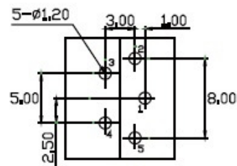
Recommended PCB Layout (PCB TOLERANCE ±0.05)
