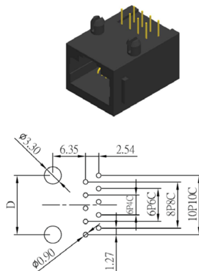
Recommended PCB Layout (PCB TOLERANCE ±0.05)
