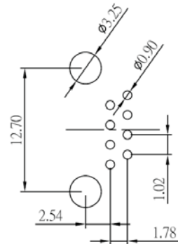
Recommended PCB Layout (PCB TOLERANCE ±0.05)
