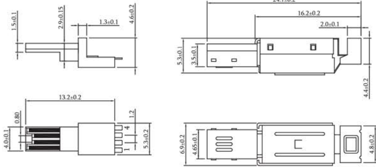
Part No.:MUSB-M4S-BB-L
