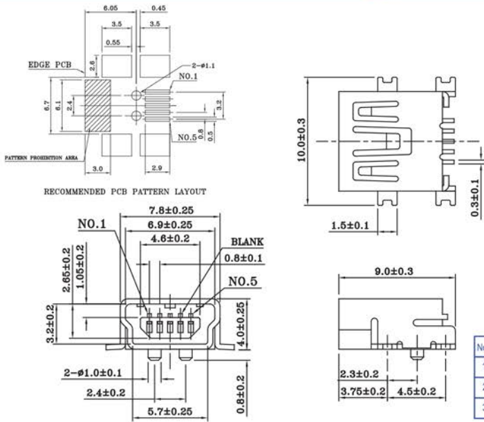
Part No.:MUSB-BS-5-U
