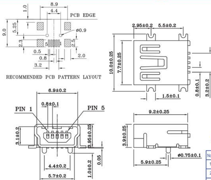
Part No.:MUSB-BS-5B-U
