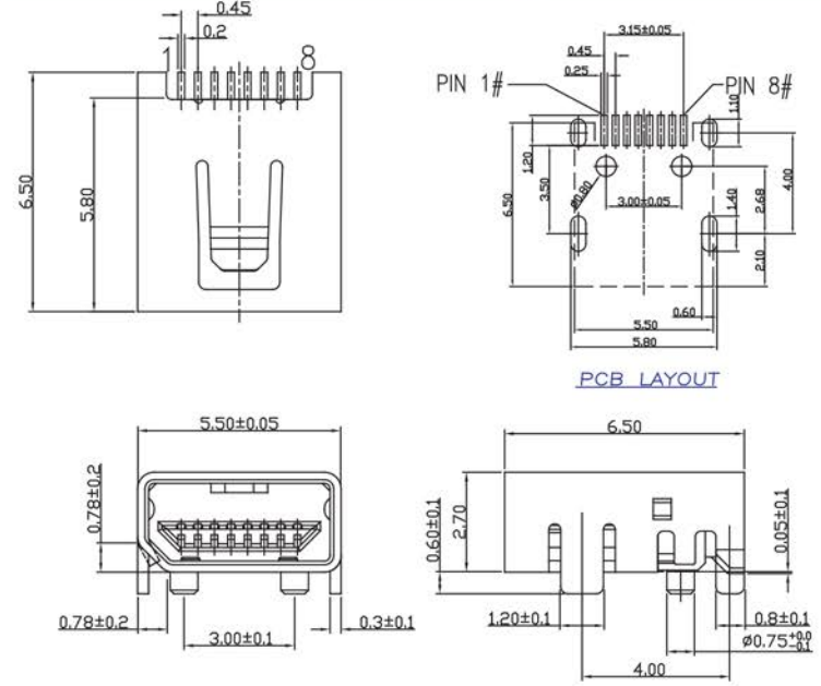
Part No.:MUSB-F108M-U
