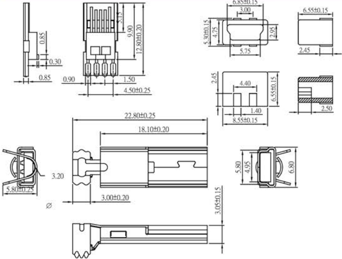
Part No.:MUSB-M5S-BB-L
