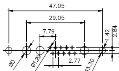
PCB LAYOUT
