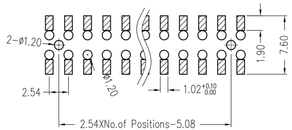
Recommended P.C.B Layout(Top Side) (PCB BOARD TOLERANCE±0.05)
